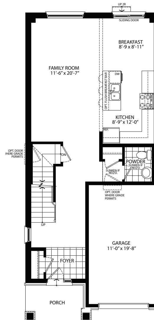
Main Floor Elevation A
