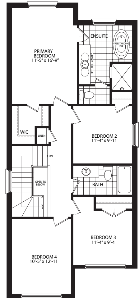
Second Floor With 4 Bedroom Option Elevation A
