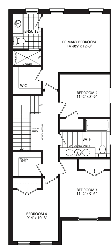
Second Floor With 4 Bedroom Option Elevation A
