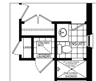
Second Floor With 4 Bedroom Option With Laundry Elevation A/B
