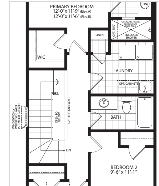
Second Floor With Laundry Option Elevation A/B
